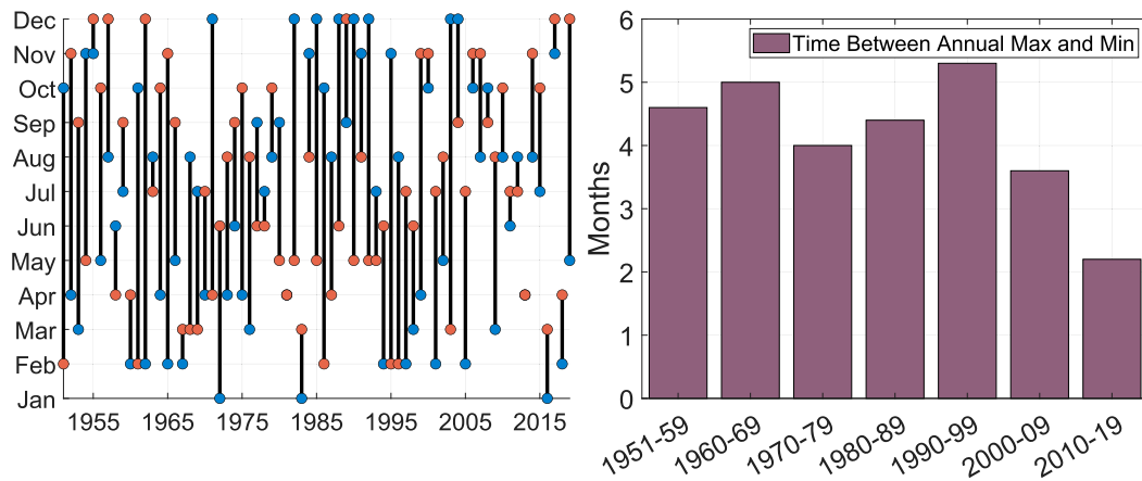
FIG. 7. (left) Points show the month of occurrence of the (red) annual minimum and (blue) annual maximum 30-day SPI in Chicago, Illinois. The black lines connect the end points and indicate the number of months elapsed between annual extremes. (right) The 10-yr average intra-annual transition duration (in months) in Chicago, Illinois.
