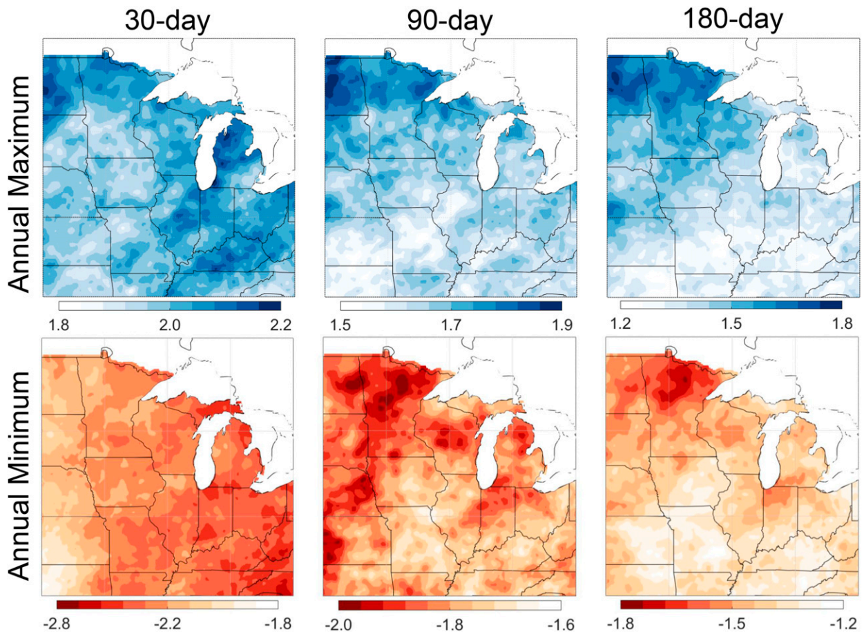
FIG. 2. Maps show the climatological (1951–2019) average annual (top) maximum and (bottom) minimum SPI across the Midwest. From left to right columns show 30-, 90-, and 180-day SPI, and color map ranges differ between the SPI durations.
