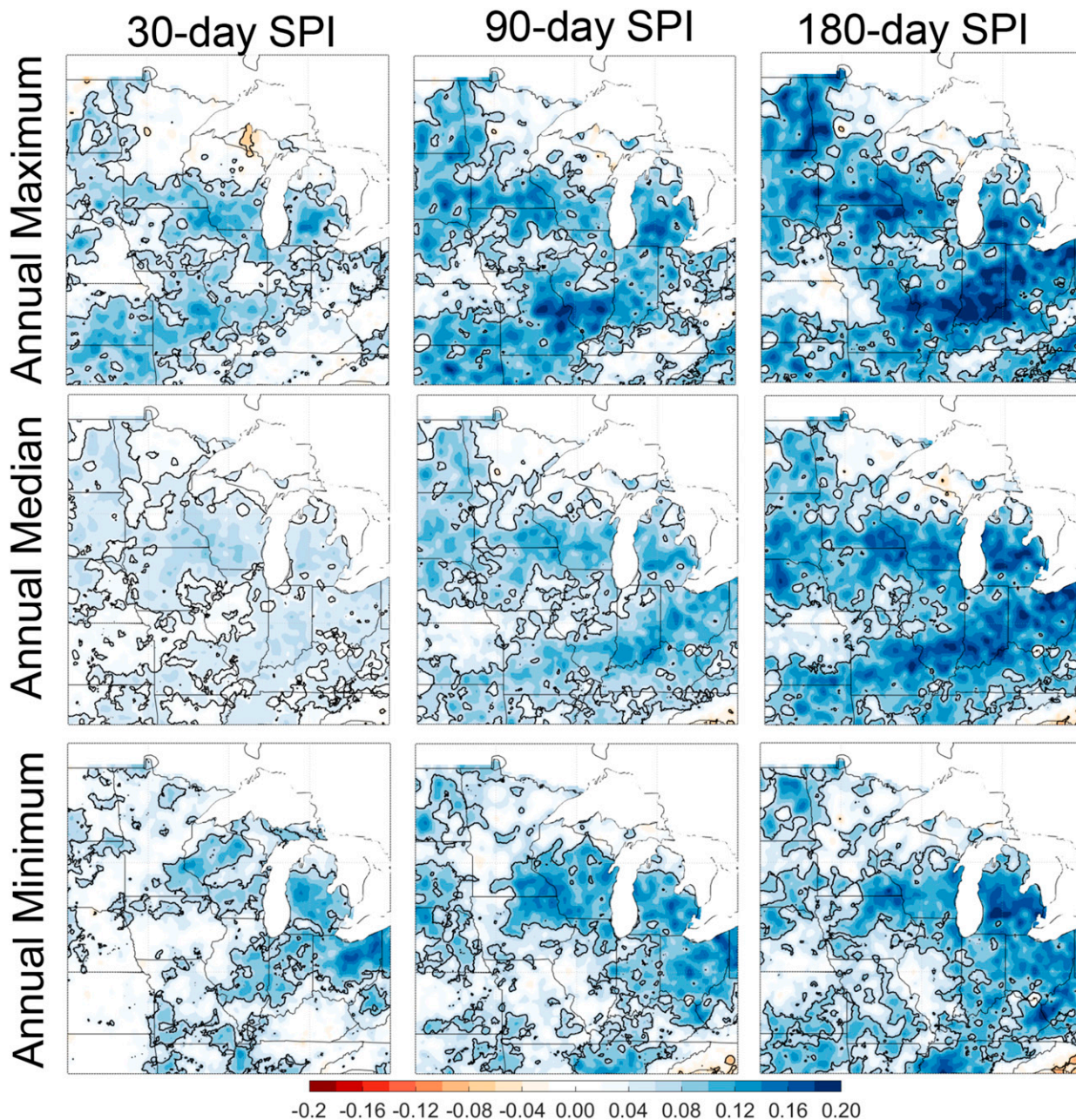
FIG. 3. Maps show (left) 30-, (center) 90-, and (right) 180-day SPI trends (change per decade) across the Midwest, calculated from 1951 to 2019. Trends are shown for (top) annual maximum, (middle) annual median, and (bottom) annual minimum SPI. Black contours indicate areas with trends that are statistically significant.
