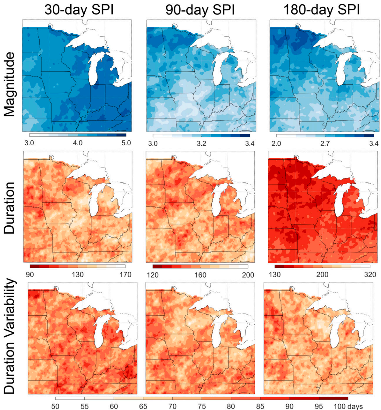
FIG. 4. Maps show climatological average intra-annual variability (top) magnitude, (middle) duration, and (bottom) duration variability. Magnitude is shown in SPI units, and duration is in units of days. Averages are computed over the period 1951–2019.
