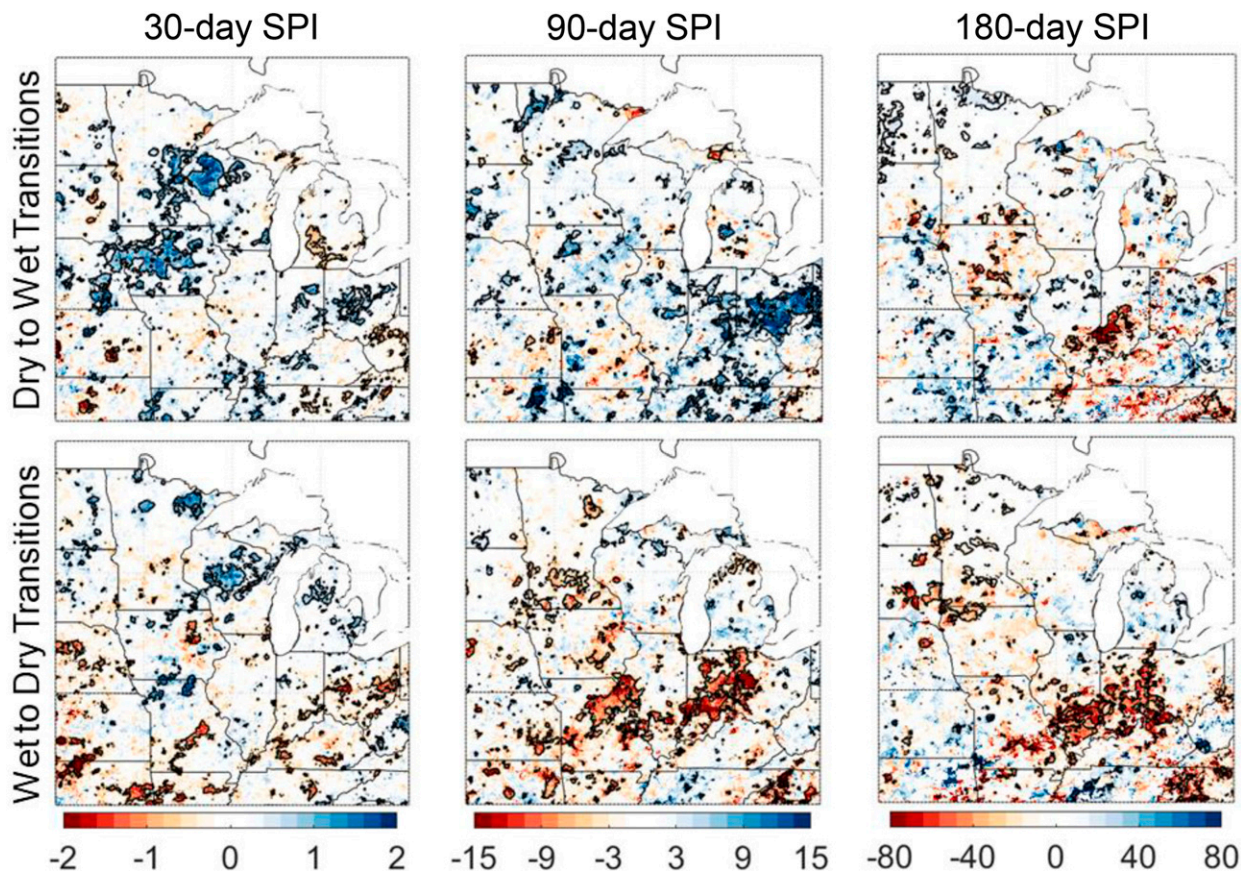
FIG. 9. Interannual transition duration trends (days per decade), calculated from 1951 to 2019. Trends are shown for (left) 30-, (center) 90-, and (right) 180-day SPI. The black contours denote areas with statistically significant duration trends.
