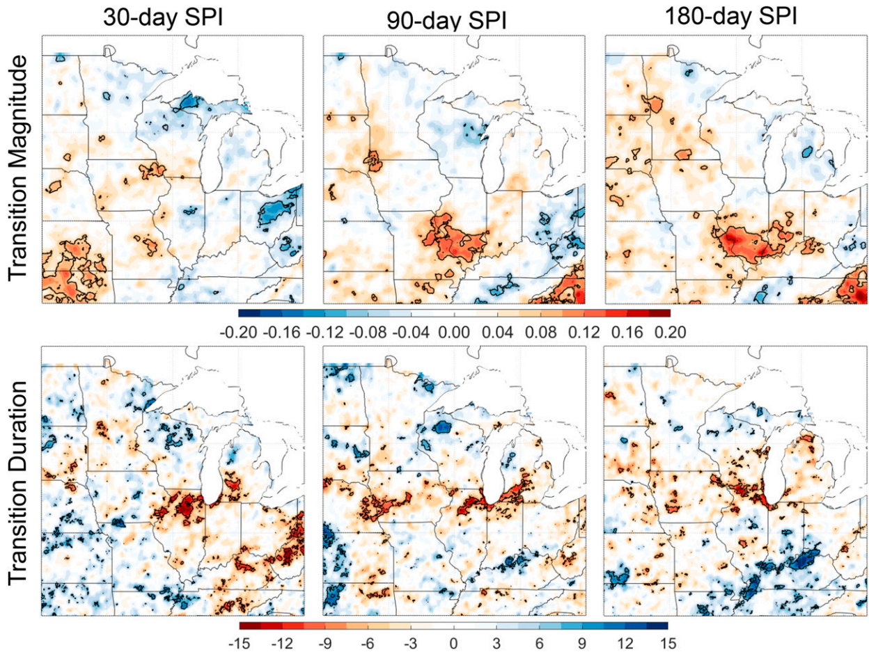
FIG. 5. Maps show trends in (top) intra-annual variability magnitude and (bottom) transition duration. Magnitude units are in change in SPI per decade, and duration trends are shown as days per decade. Black contours highlight areas with statistically significant trends.
