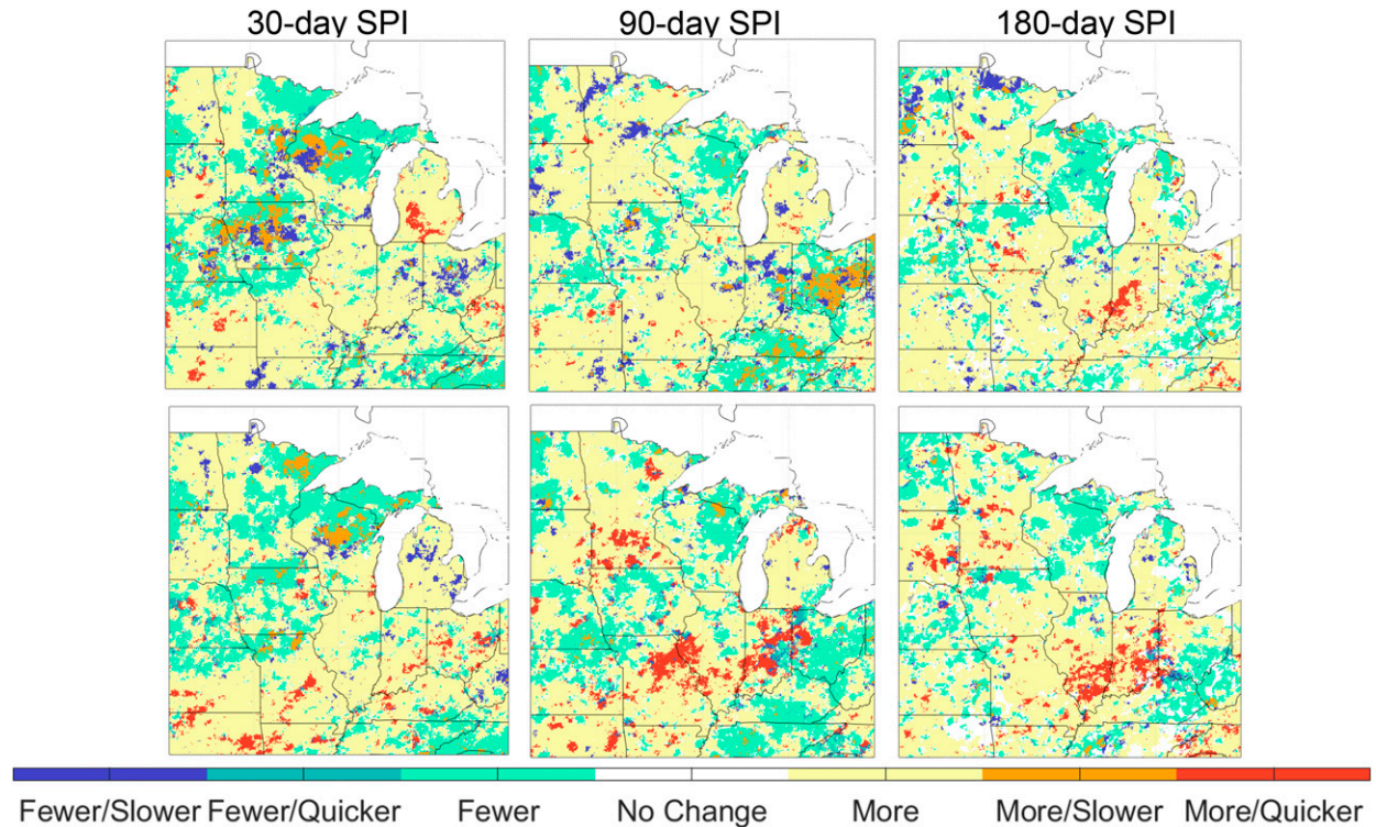
FIG. 10. Areas are colored depending on the joint change in interannual transition duration and frequency. Areas in which transitions are denoted as happening “quicker” are those with statistically significant, negative duration trends.
