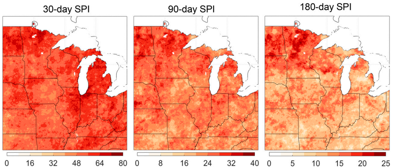
FIG. 8. Climatological (1951–2019) interannual transition frequency in (left) 30-, (center) 90-, and (right) 180-day SPI.
