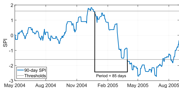
FIG. 1. Example of interannual transition in precipitation extremes. Blue line shows 90-day SPI between May 2004 and August 2005 in Peoria, Illinois (40.69°N, 89.59°W). The black lines indicate the transition start and end, with an overall duration of 85 days.
