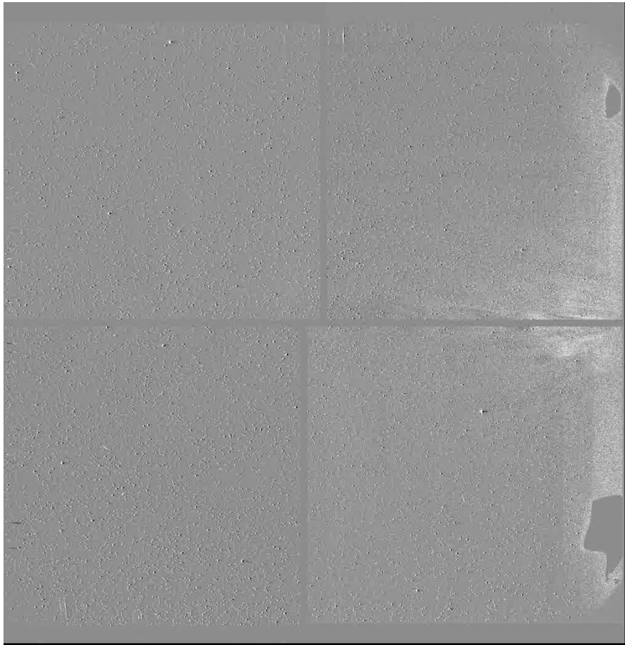
SoloHI Mosaic Feb 23 2021
