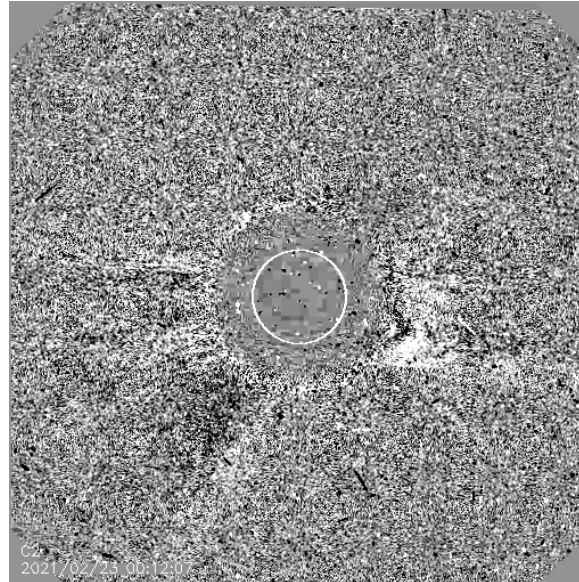
LASCO C2
