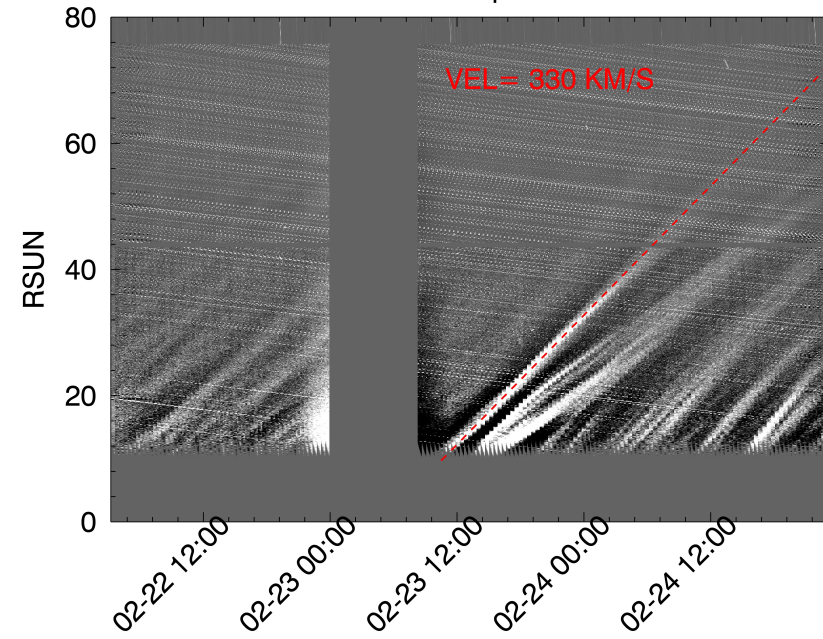
SoloHI J-Map PA=88
