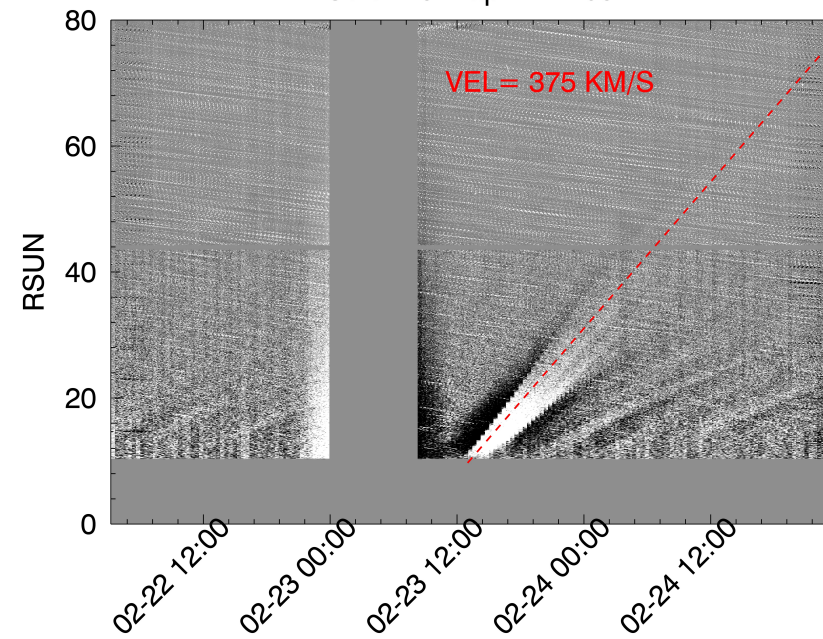
SoloHI J-Map PA=108
