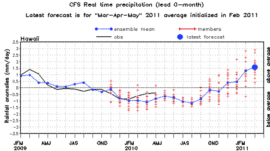
The average deviation from climatology rainfall in mm/day for the period "Mar-Apr-May" 2011 as predicted by the ensemble means (large blue dot) and by the 15-ensemble members (red crosses) of the model that was initialized in Feb 2011. Past 0-month lead forecasts are also shown to illustrate the models forecast skill. Quality control observations (solid black line) are available only through June 2010. Each tick mark represents a 3-month period.
