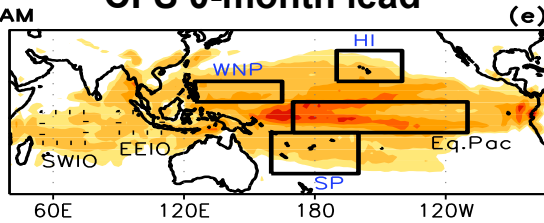
CFS 0-month lead
