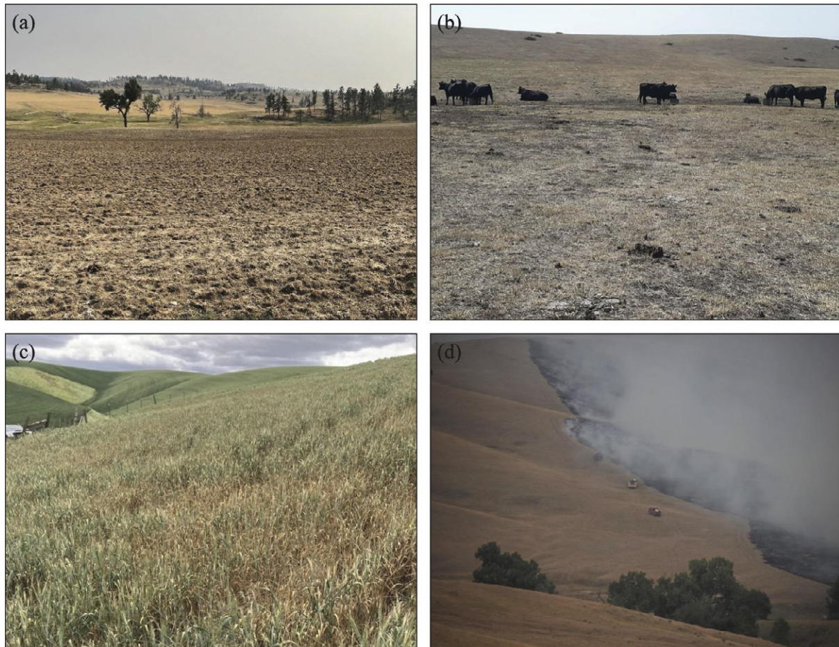
Fig. 1. Pictures showing the diverse impacts of flash drought during 2021, including (a) spring wheat in central Montana that did not have enough rain to germinate by 09 August, (b) heavily grazed pasture in central Montana on 07 September, (c) poor winter wheat heading in southeastern Washington on 21 May, and (d) a grassfire in central South Dakota on 02 August. All pictures were obtained from the Condition Monitoring Observer Report for Drought (CMOR-Drought) tool maintained by the National Drought Mitigation Center.
