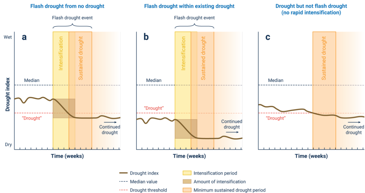
Fig. 2. Idealized time series showing the evolution of a generic drought monitoring index for: (a) flash drought development from a drought-free initial state, (b) flash drought development during an ongoing drought, and (c) slow intensification during conventional drought. Time increments along the x-axis are notional, with agricultural flash drought used in this example to demonstrate the flash drought identification framework. Yellow shading depicts the period of rapid intensification whereas the orange shading denotes the minimum length of time that drought must persist for an event to be considered flash drought. Note that the lengths of the intensification and minimum drought periods shown here are for illustrative purposes and can be adjusted to accommodate the emergence of different impacts or the needs of different practitioners.
